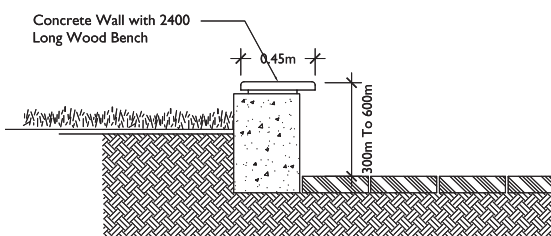
SEATING TYPE 3: Wooden seating strip fixed on top of concrete retaining wall
