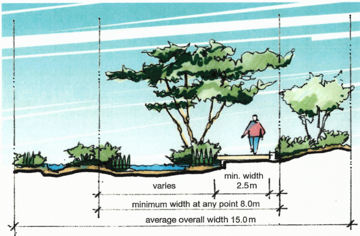
FIGURE 13: Illustrative Section across Internal Greenway (Illustrating key dimensions)
